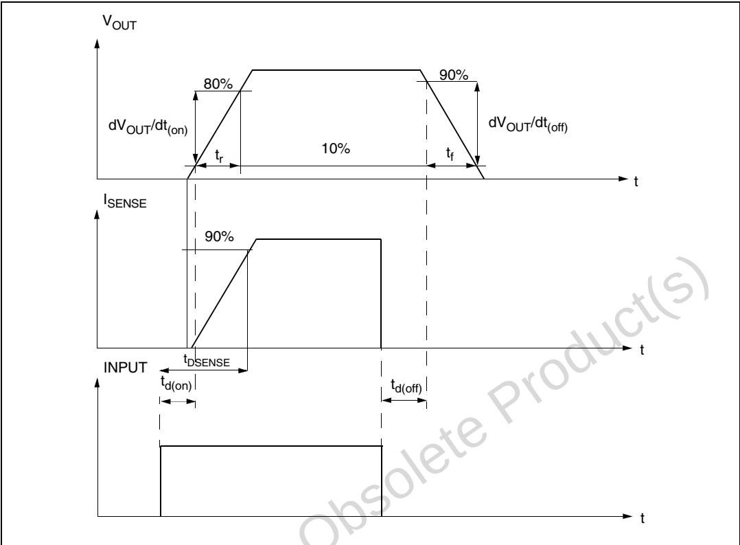
Figure 5. Switching characteristics
