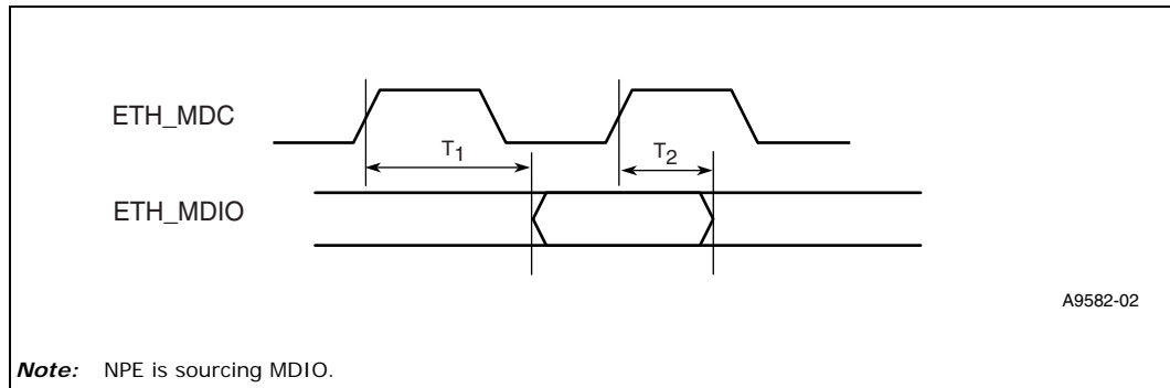
Figure 21. MDIO Output Timings
