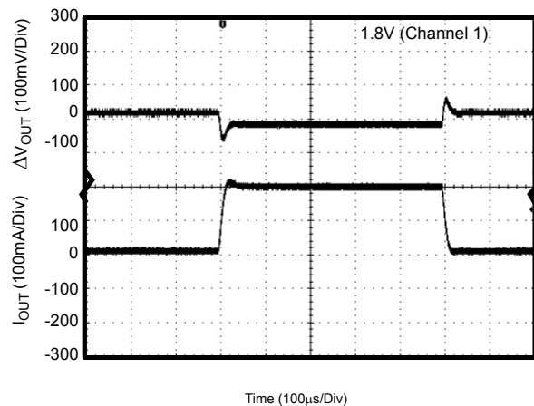
Figure 37. Load Transient (Conditions: I_{OUT}=10 to 200mA , C_{IN}=C_{OUT}=1\mu F )
