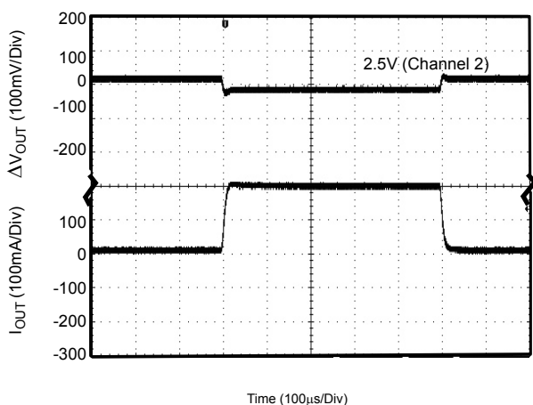
Figure 38. Load Transient (Conditions: I_{OUT}=10 to 200mA , C_{IN}=C_{OUT}=1\mu F )
