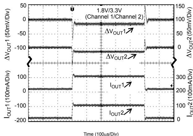
Figure 49. Cross Talk 9
