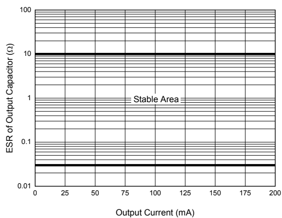
Figure 51. ESR vs. Output Current
