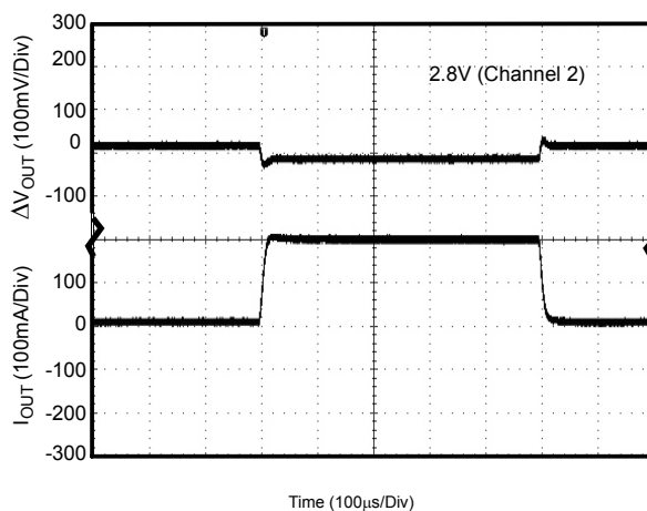
Figure 39. Load Transient (Conditions: I_{OUT}=10 to 200mA , C_{IN}=C_{OUT}=1\mu F )
