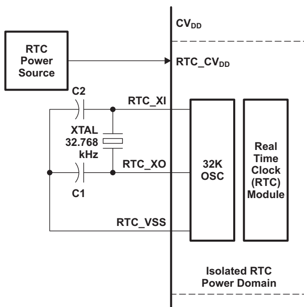
Figure 6-83. Clock Source
