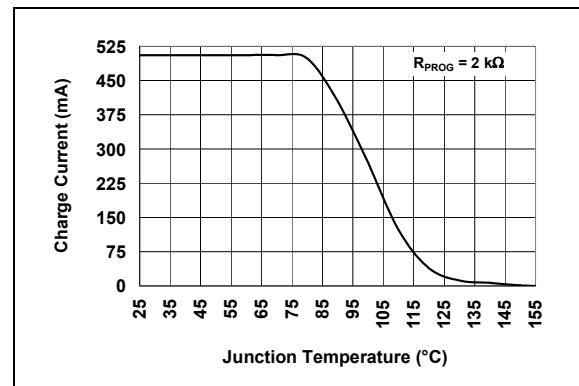
FIGURE 4-2: Thermal Regulation.
