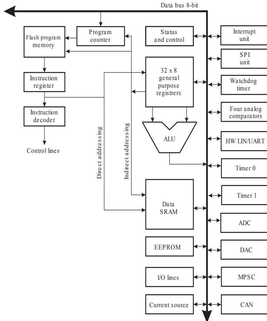
Figure 3-1. Block diagram.
