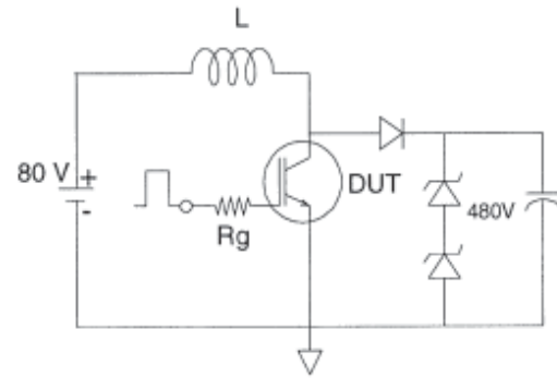
Fig.C.T.2 - RBSOA Circuit
