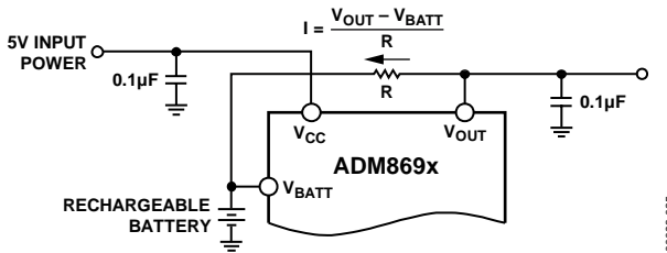
Figure 25. Rechargeable Battery
