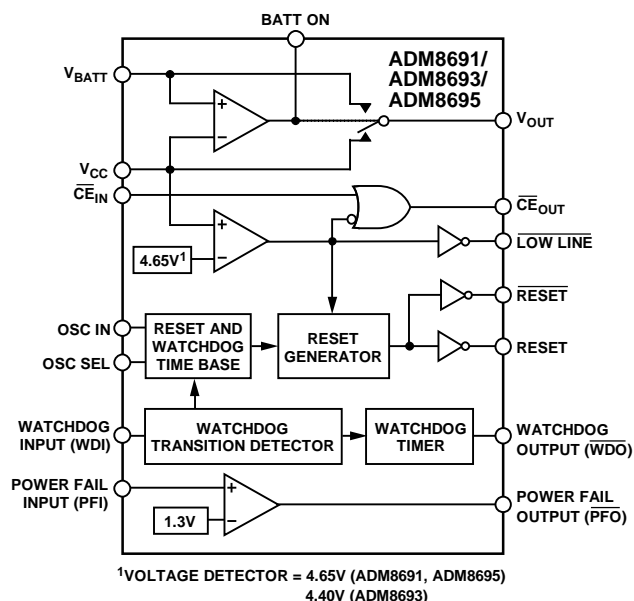
Figure 2. ADM8691/ADM8693/ADM8695
