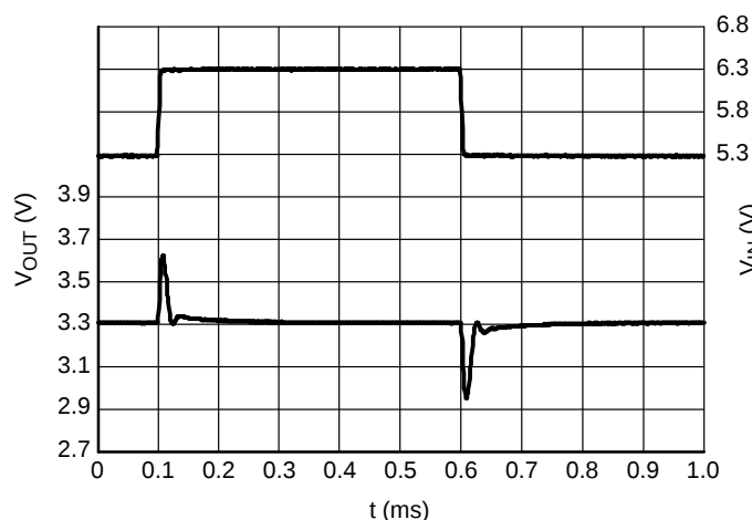
Figure 31. Line Transients, 3.3 V Version, t_R = t_F = 5 \mu\text{s} , I_{OUT} = 30 \text{ mA}
