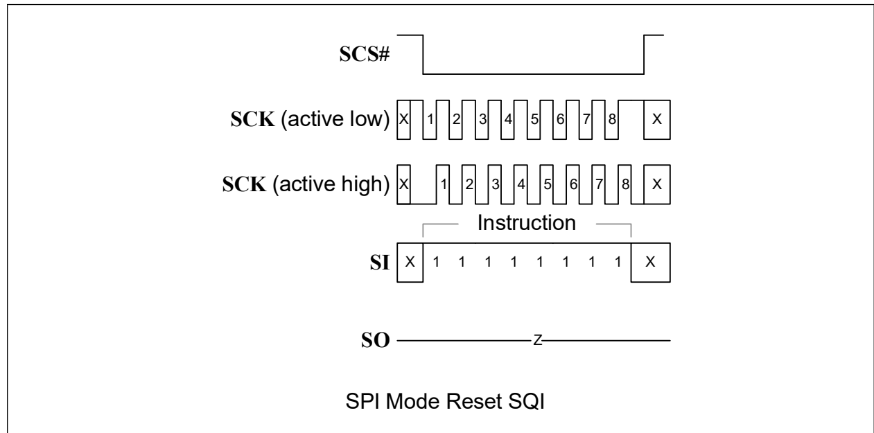
FIGURE 9-4: SPI MODE RESET SQI
