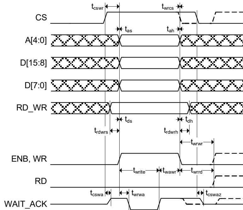
FIGURE 8-60: INDEXED ADDRESSING NON-POSTED WRITE CYCLE TIMING
