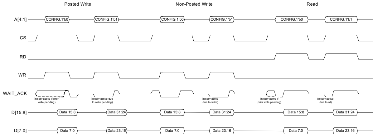
FIGURE 8-45: INDEXED ADDRESSING CONFIGURATION REGISTER ACCESS - 16-BIT POSTED WRITE / NON-POSTED WRITE / READ
