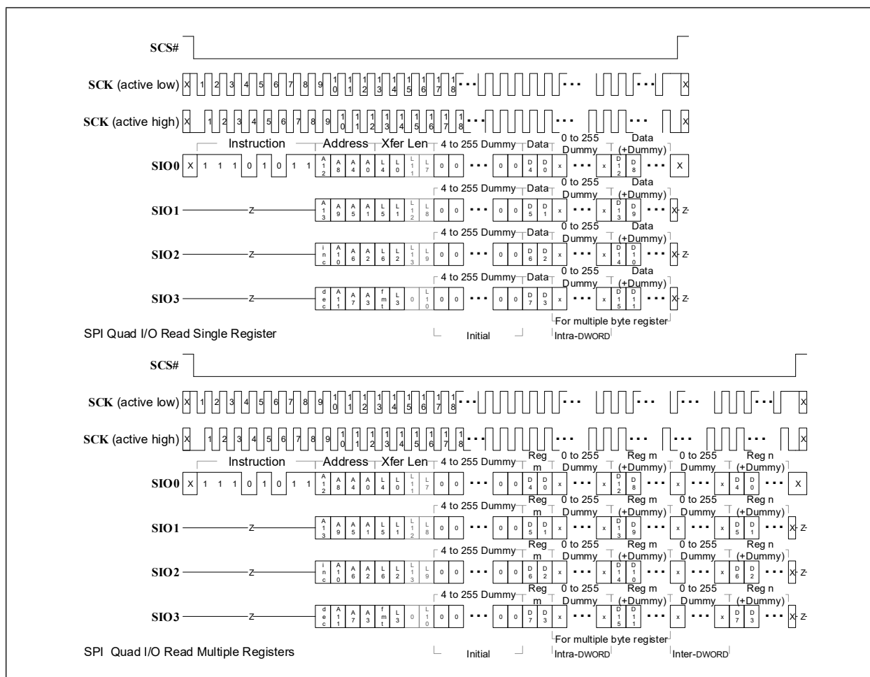
FIGURE 9-12: SPI QUAD I/O READ
