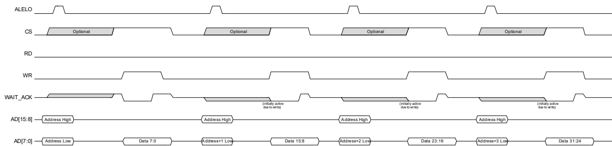
FIGURE 8-44: MULTIPLYING ADDRESSING WITH SINGLE PHASE LATCHING - 8-BIT NON-POSTED WRITE
