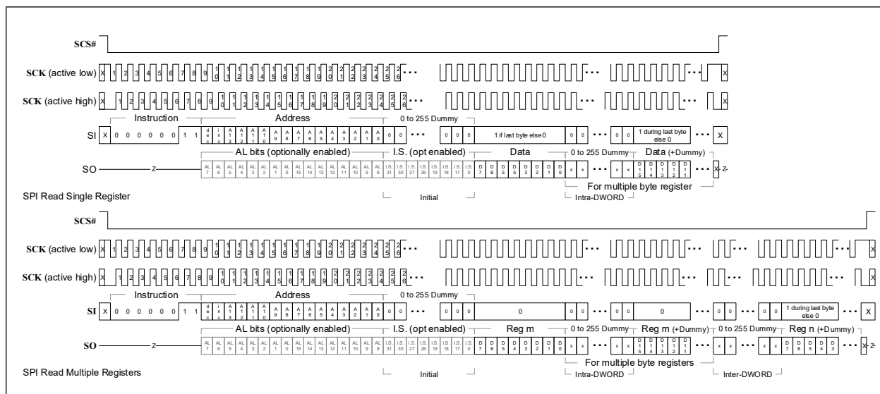
FIGURE 9-6: SPI READ
