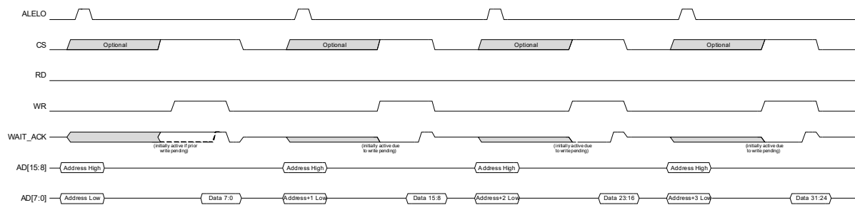
FIGURE 8-43: MULTIPLEXED ADDRESSING WITH SINGLE PHASE LATCHING - 8-BIT POSTED WRITE
