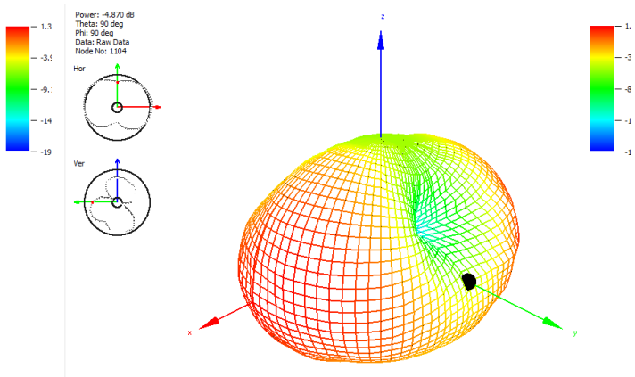
2000 MHz
