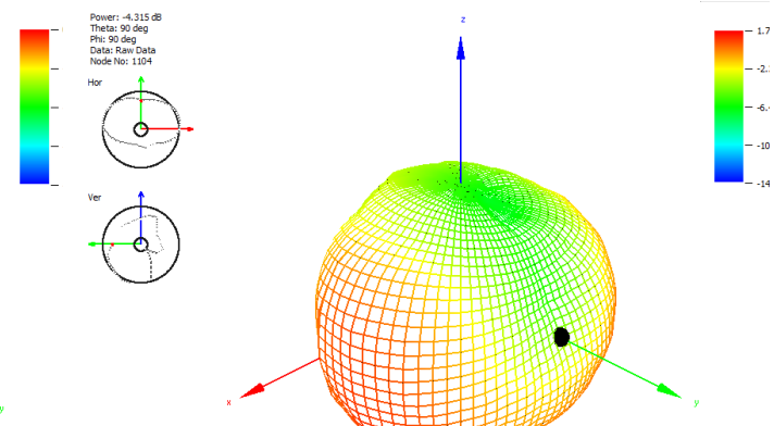
1750 MHz
