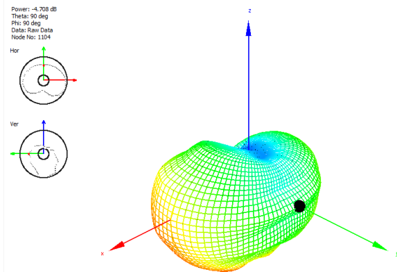
700 MHz
