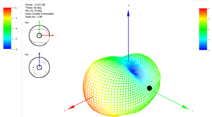
850 MHz
