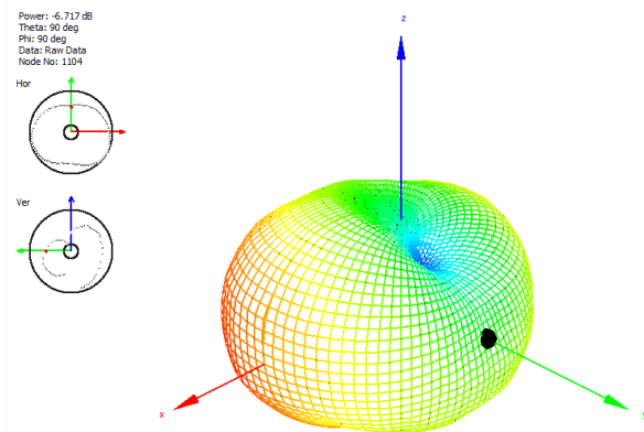
950 MHz
