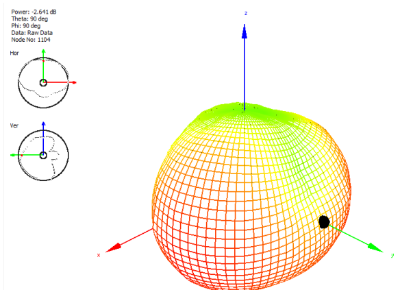
1850 MHz
