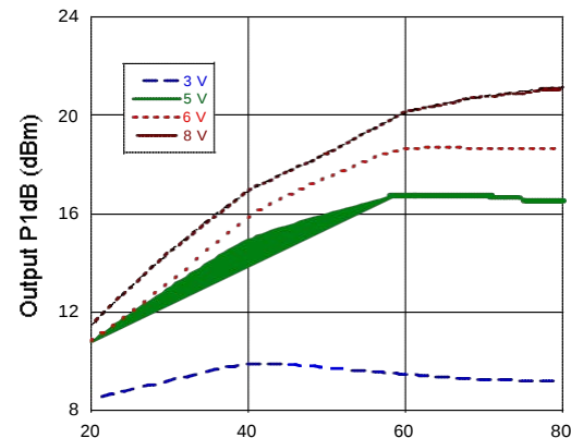
Output P1dB vs. Current, F = 900\ \text{MHz}
