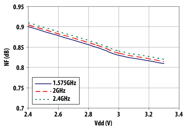
Figure 4. NF vs Vdd vs Freq
