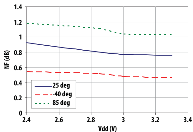
Figure 9. NF vs Vdd vs Temp
