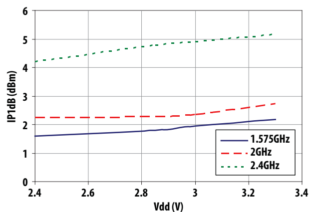
Figure 6. IP1dB vs Vdd vs Freq
