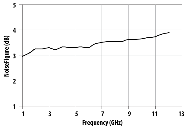
Figure 2. Noise Figure [1]
