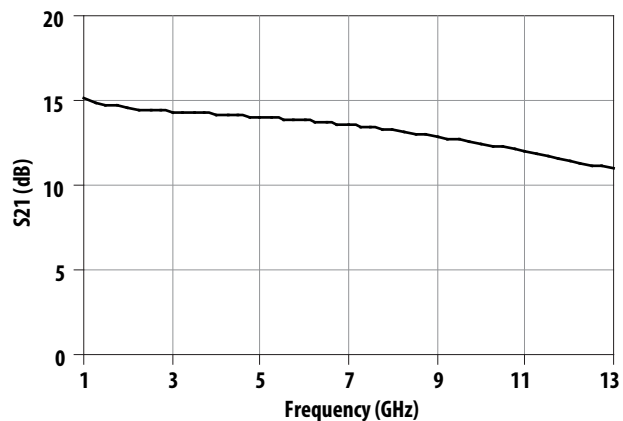
Figure 1. Small-signal Gain [1]
