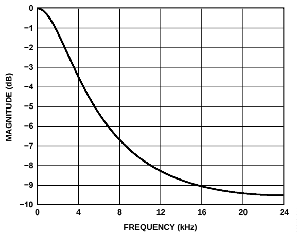
Figure 15. De-Emphasis Frequency Response, Audio Sampling Rate = 48 kHz
