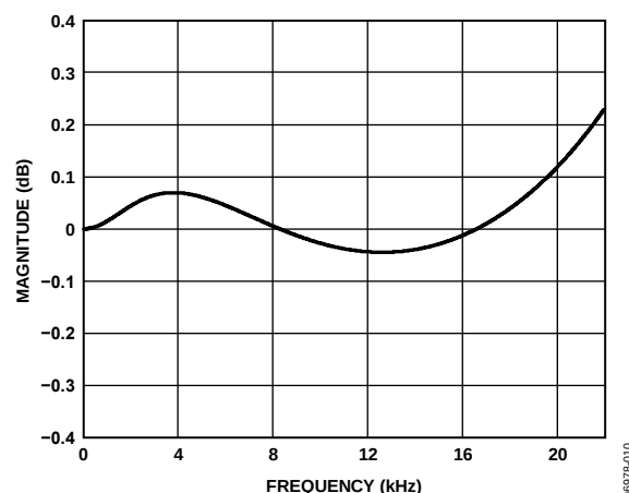
Figure 14. De-Emphasis Error, Audio Sampling Rate = 44.1 kHz
