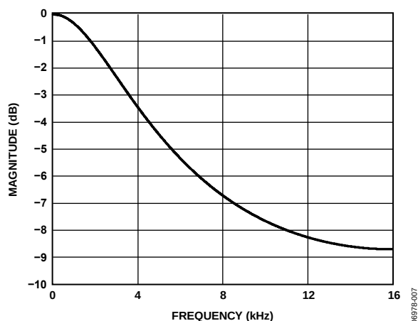
Figure 11. De-Emphasis Frequency Response, Audio Sampling Rate = 32 kHz
