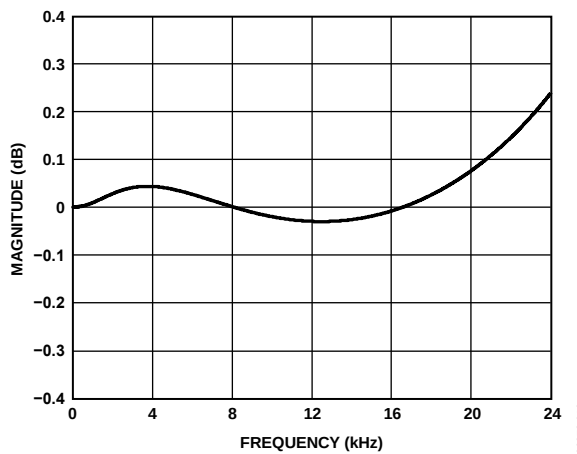
Figure 16. De-Emphasis Error, Audio Sampling Rate = 48 kHz
