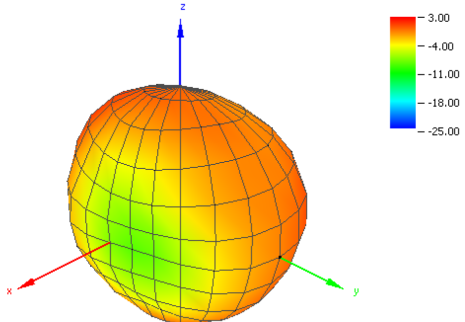
Figure 10. Radiation Pattern at 1400 MHz of FXUB63 Antenna.
