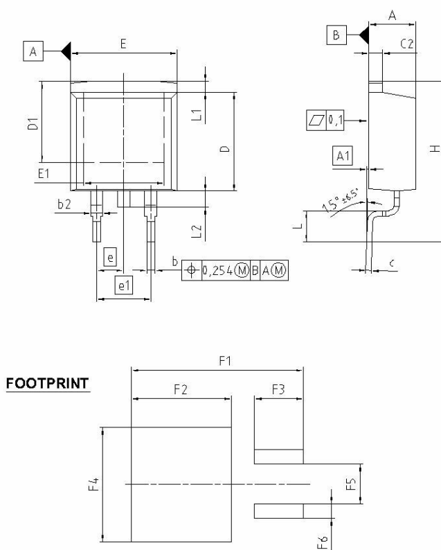
PG-TO263-3-2
