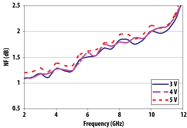
Figure 5. Noise Figure (50 ohm) over Vdd
