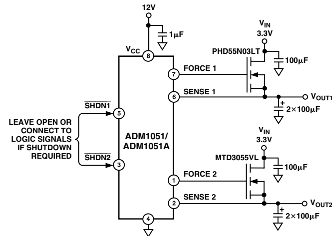
Figure 1. Test Circuit
