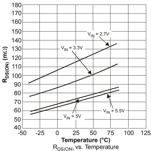
R_{\text{DS(ON)}} vs. Temperature
