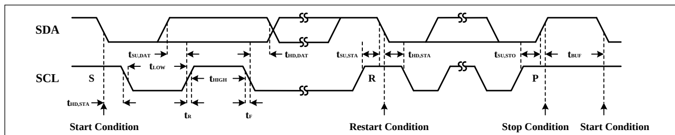
Figure 4 Interface Timing
