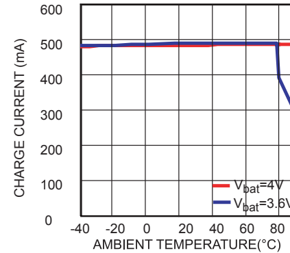
Charge Current(500mA) vs. Ambient Temperature
