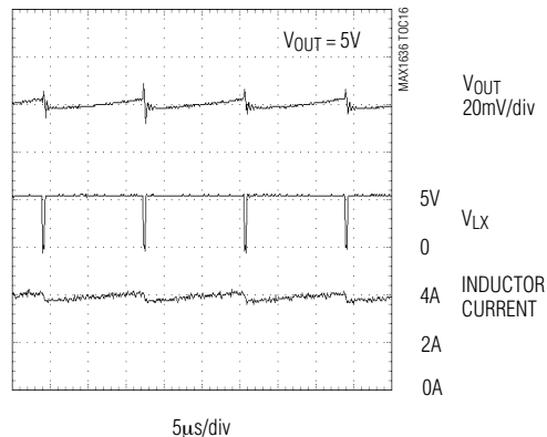
OVERVOLTAGE-PROTECTION WAVEFORMS ( V_{IN} SHORTED TO V_{OUT} THROUGH a 0.5\Omega RESISTOR)
