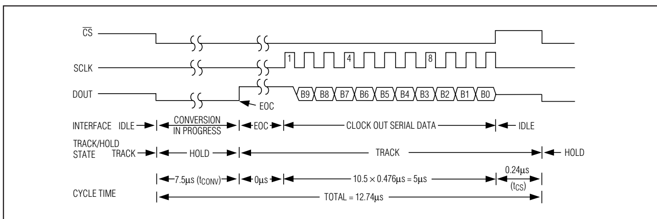
Figure 8b. Interface Timing Sequence—Minimum Cycle Time
