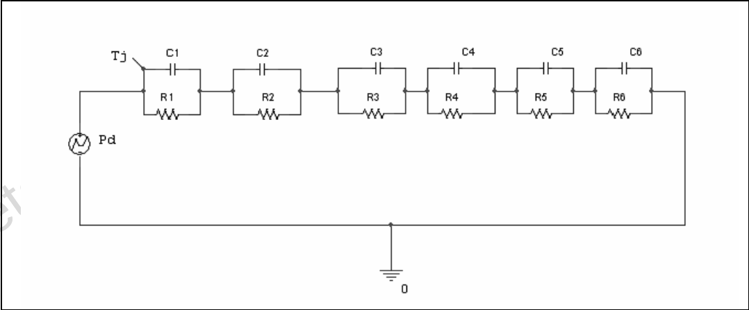
Figure 12. PowerSSO-12 thermal fitting model of a single channel
