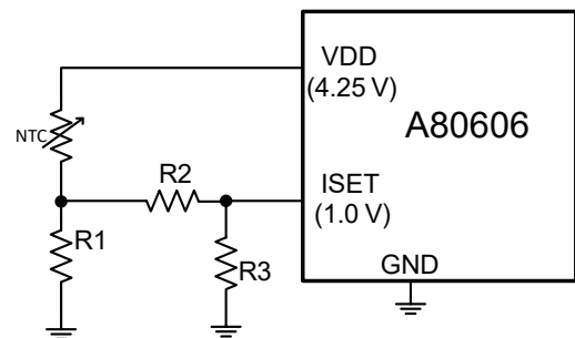
Figure 31: Thermal foldback of LED current using NTC thermistor ILED VS Temperature with NTC Circuit
