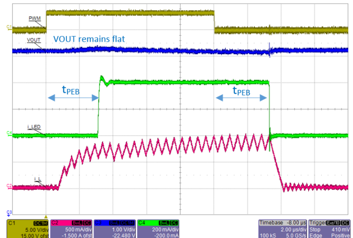
Figure 21: A80606 PWM dimming operation with PEB delay set to 3 \mu s. Note that V_{OUT} ripple is reduced to ~0.2 V.
