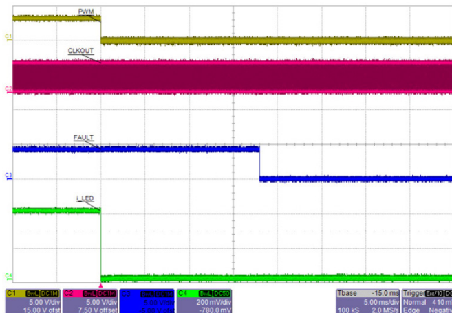
Figure 34: As long as EN = H, the IC does not shut down VDD and CLKOUT. But internal latched faults are cleared by PWM = L for ~16 ms.
