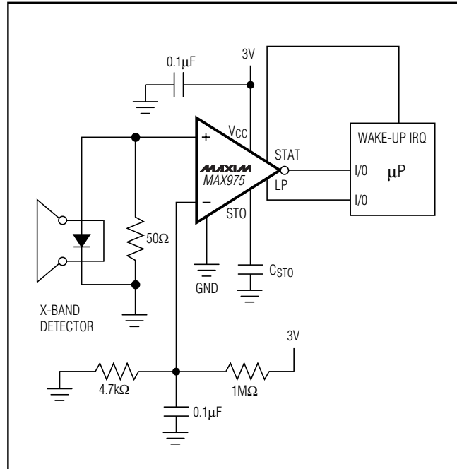
Figure 6. Toll-Tag Reader
