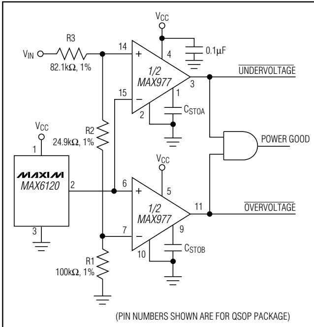
Figure 5. Window Comparator
