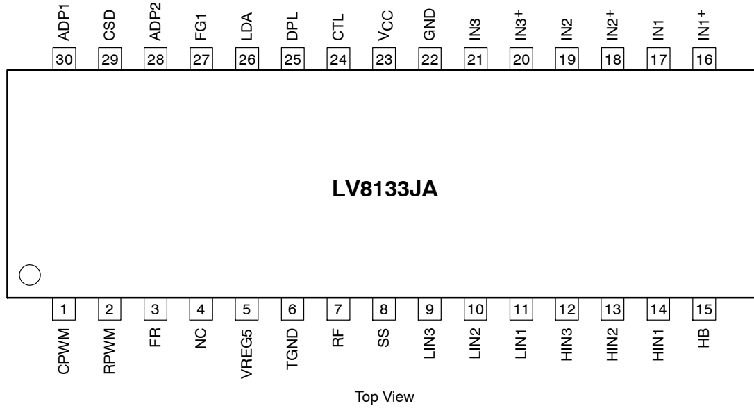
Figure 4. Pin Assignment
