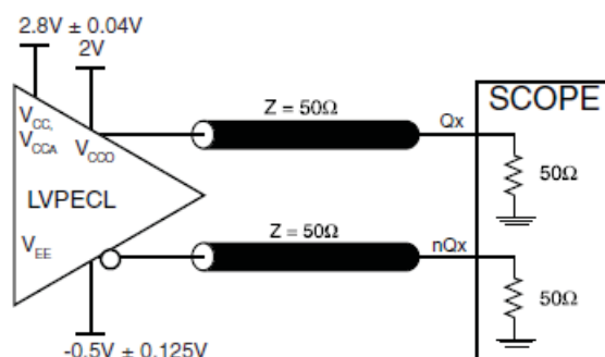
3.3V/2.5V OUTPUT LOAD AC TEST CIRCUIT
