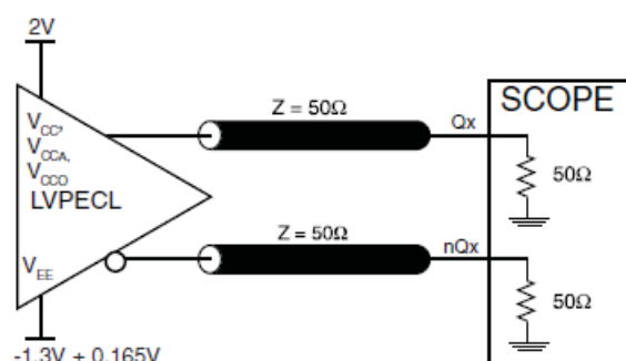
3.3V/3.3V OUTPUT LOAD AC TEST CIRCUIT
