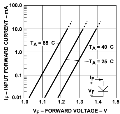
Figure 6. Typical diode input forward current characteristic.
