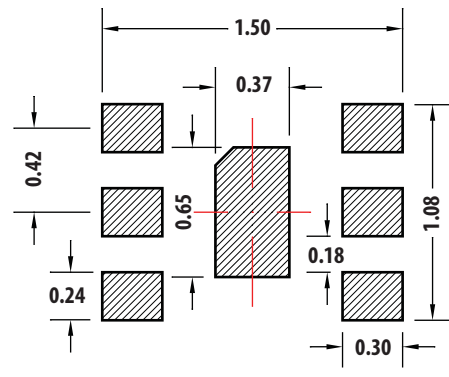
Stencil Opening
