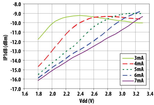
Figure 11. IP1dB vs Vdd
