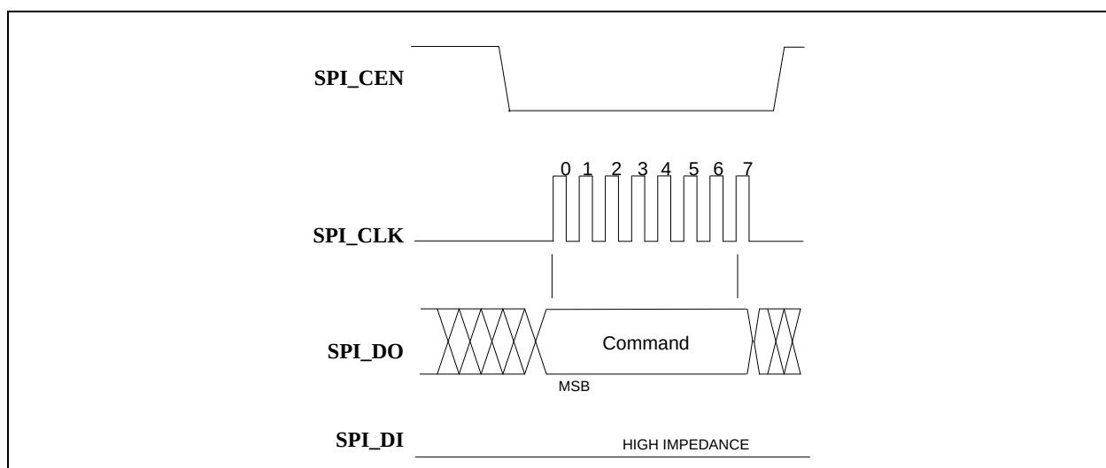
FIGURE 4-8: SPI COMMAND ONLY SEQUENCE
