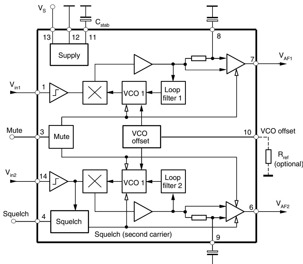
Figure 1-1. Block Diagram
