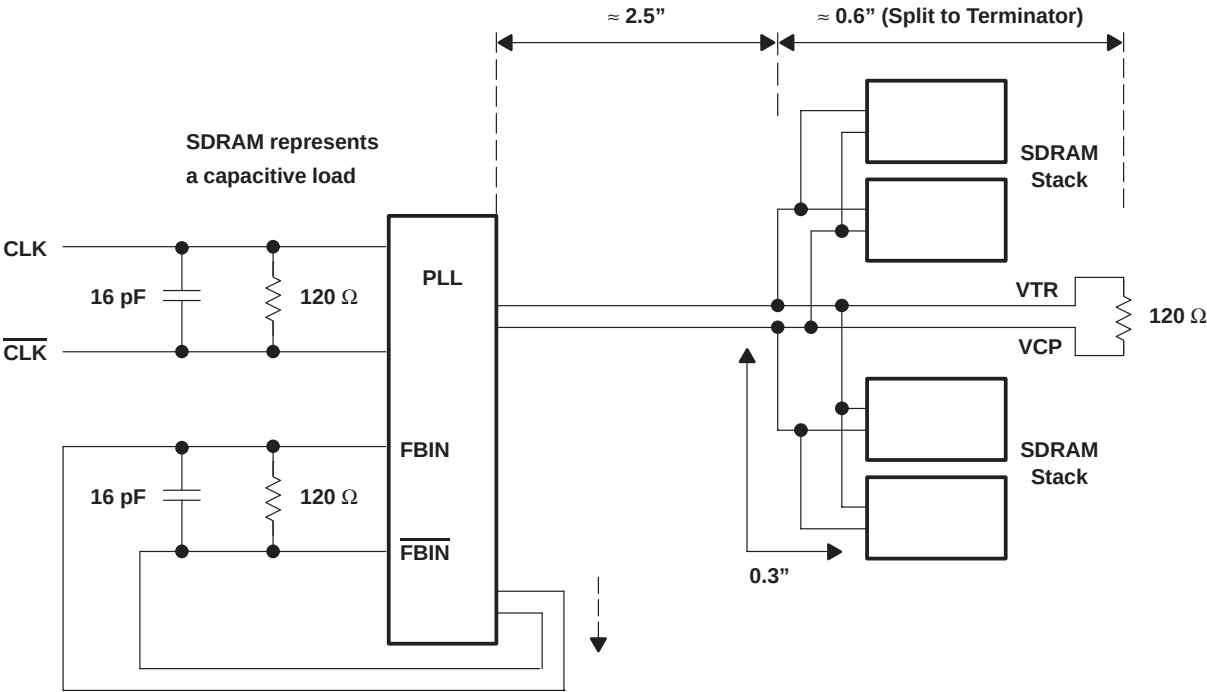
Figure 2. Clock Structure #2
