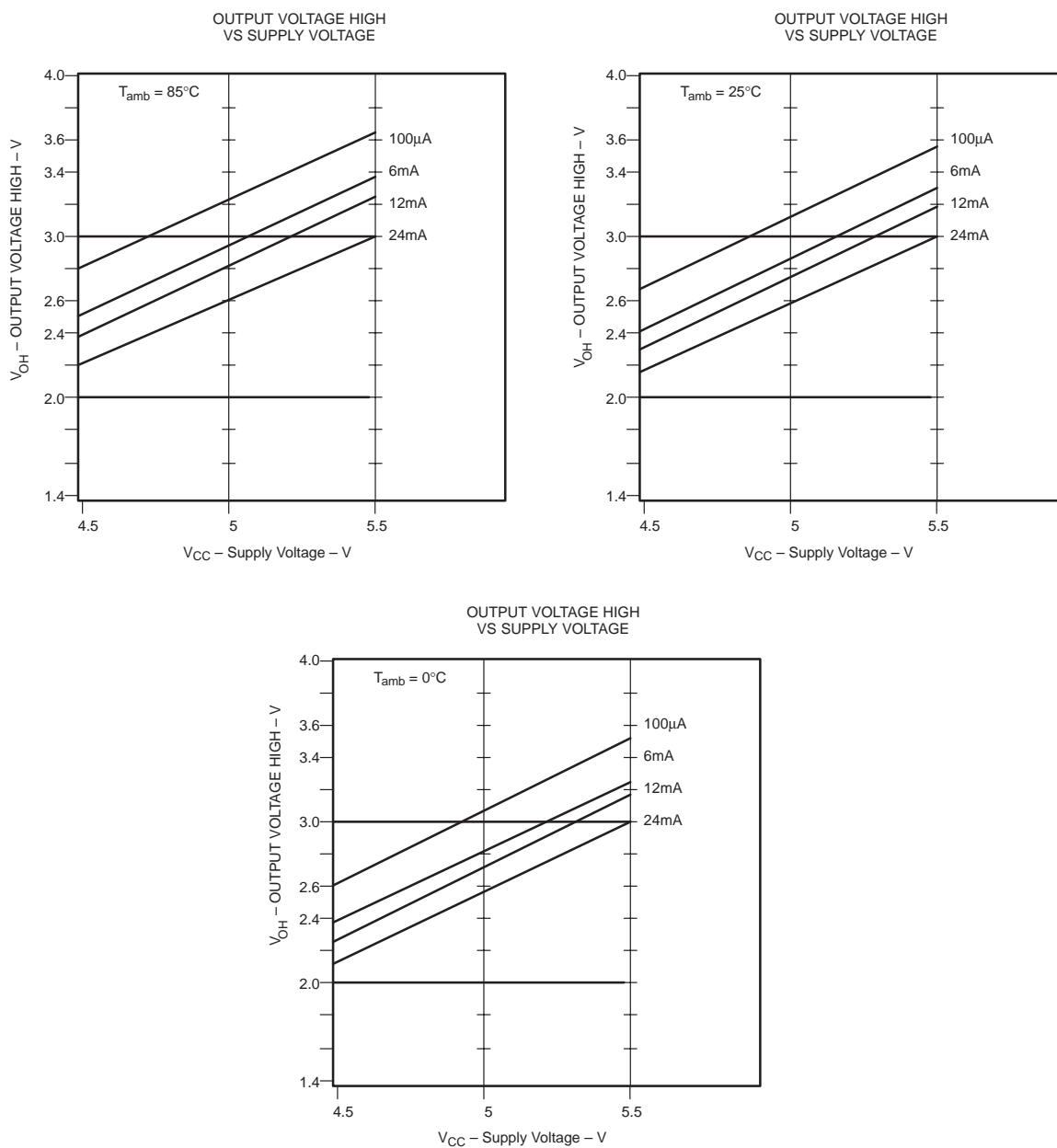
Figure 1. V_{OH} values ( V_{in} = V_{CC} )
