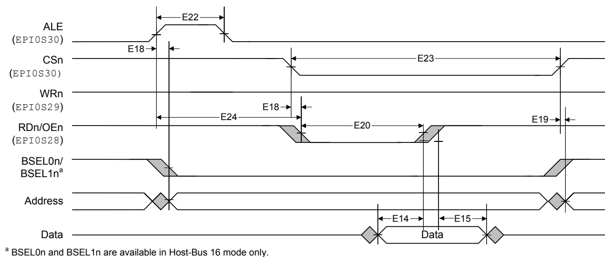
Figure 26-14. Host-Bus 8/16 Mode Read Timing
