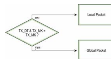
Figure 4-02. Local Packets vs. Global Packets (Transmitting Module)
