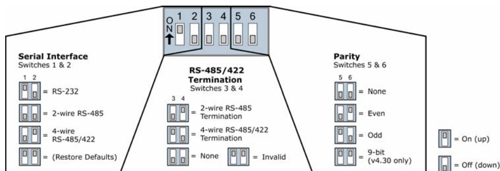
Figure B-03. MaxStream XIB-R (RS-232/485) Interface Board DIP Switch Settings
