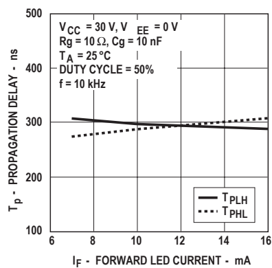
Figure 13. Propagation Delay vs. I_F .
