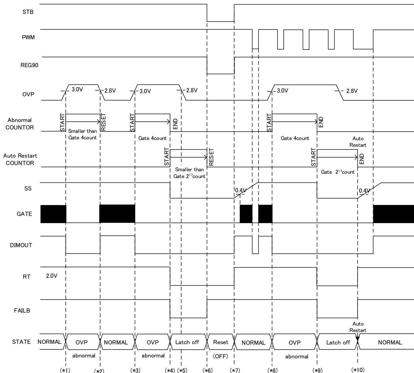
Figure 37. OVP Detection
