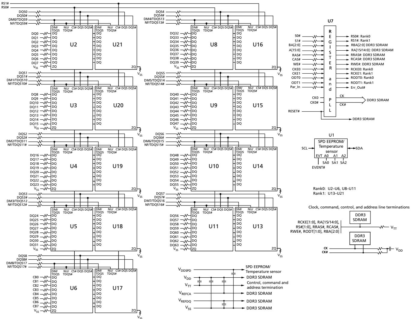
Figure 3: Functional Block Diagram R/C B1(PCB 1164 and 1560)
