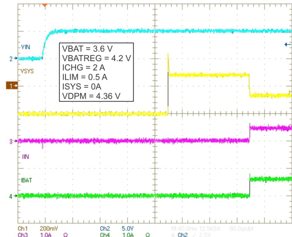
Figure 42. Start-up, 4.2 V
