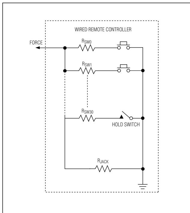
Figure 10. Software Implemented Hold-Switch Configuration
