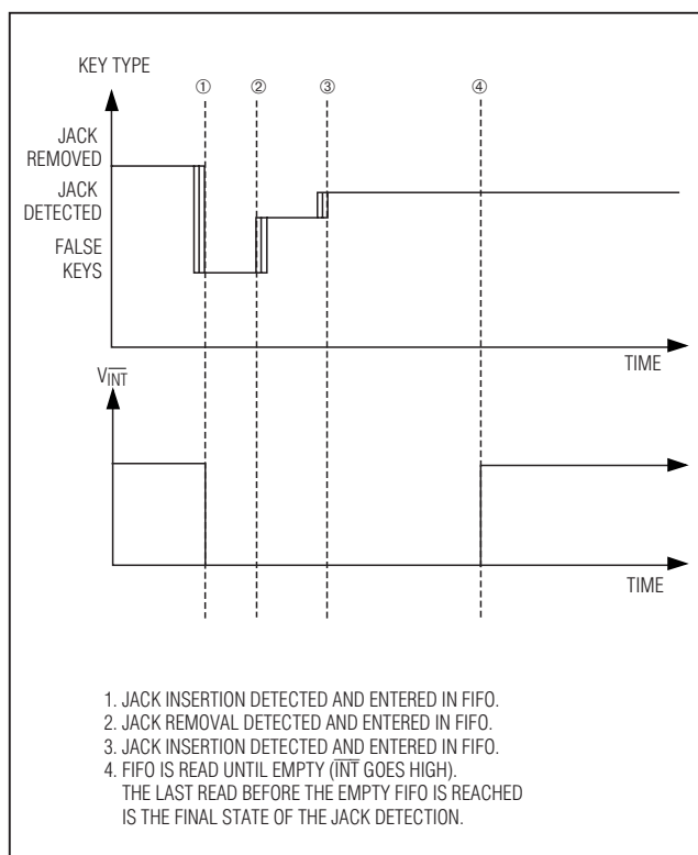
Figure 9. Jack Insertion Detection
