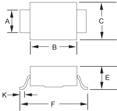
Figure 5-1. SMCG (DO-215AB)
