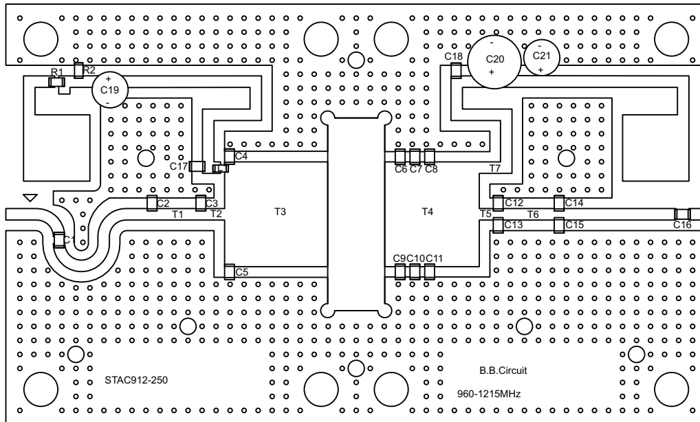
Figure 6. Broadband 960-1215 MHz circuit
