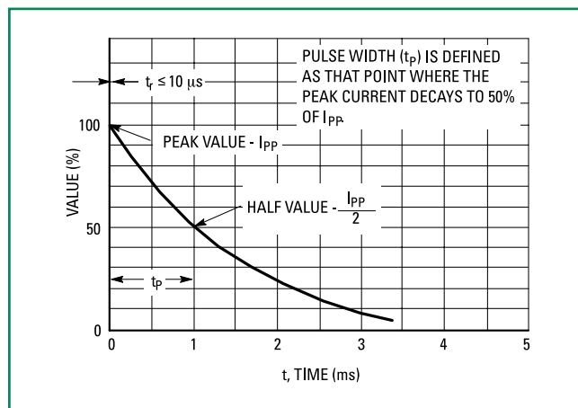
Figure 7. Pulse Waveform
