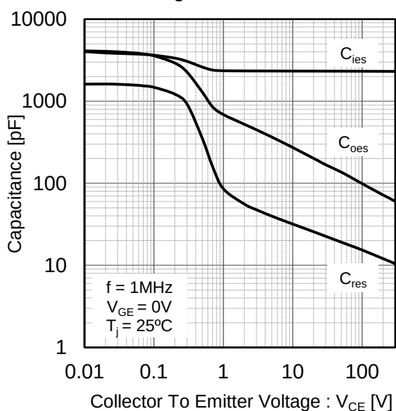
Fig.15 Typical Capacitance vs. Collector Emitter Voltage
