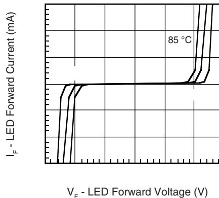
Fig. 7 - LED Forward Current vs. Forward Voltage
