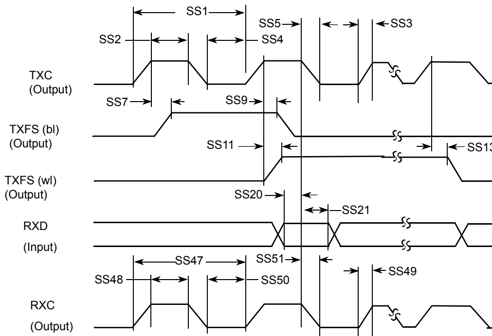
Figure 84. SSI Receiver Internal Clock Timing Diagram
