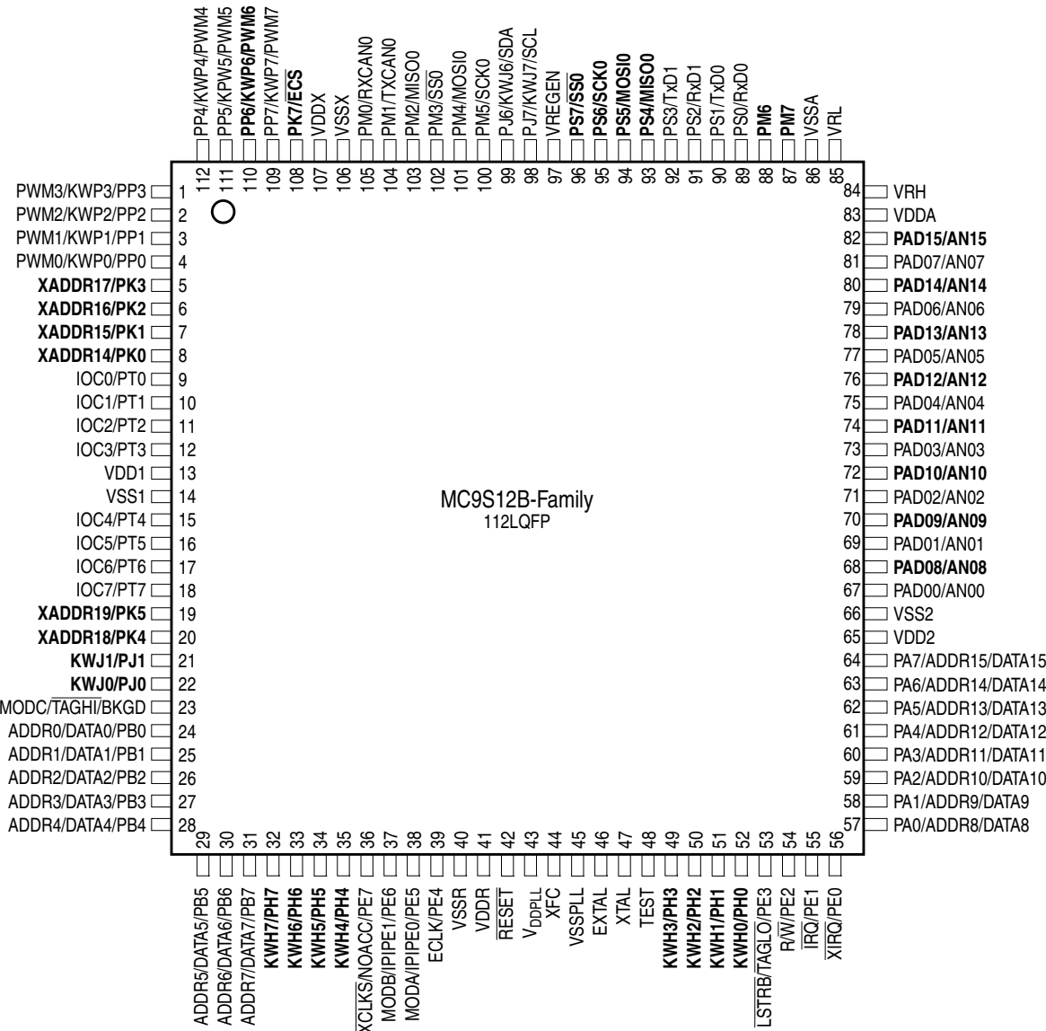
Figure 1. Pin assignments 112 QFP for MC9S12B-Family
