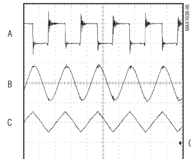
SWITCHING WAVEFORMS
