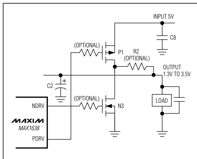
Figure 6. GlitchCatcher Circuit
